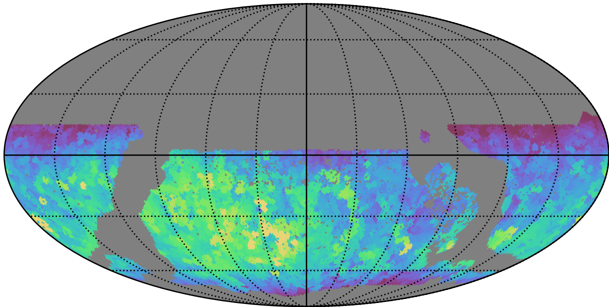
ddf_loaded_fl15_v3.4_10yrs WFD r band: Max fiveSigmaDepth
