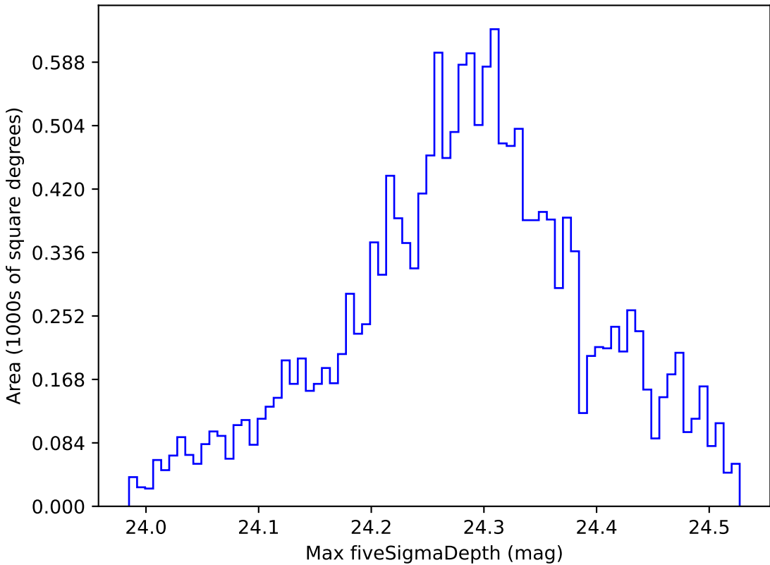
ddf_loaded_fl15_v3.4_10yrs WFD i band: Max fiveSigmaDepth
