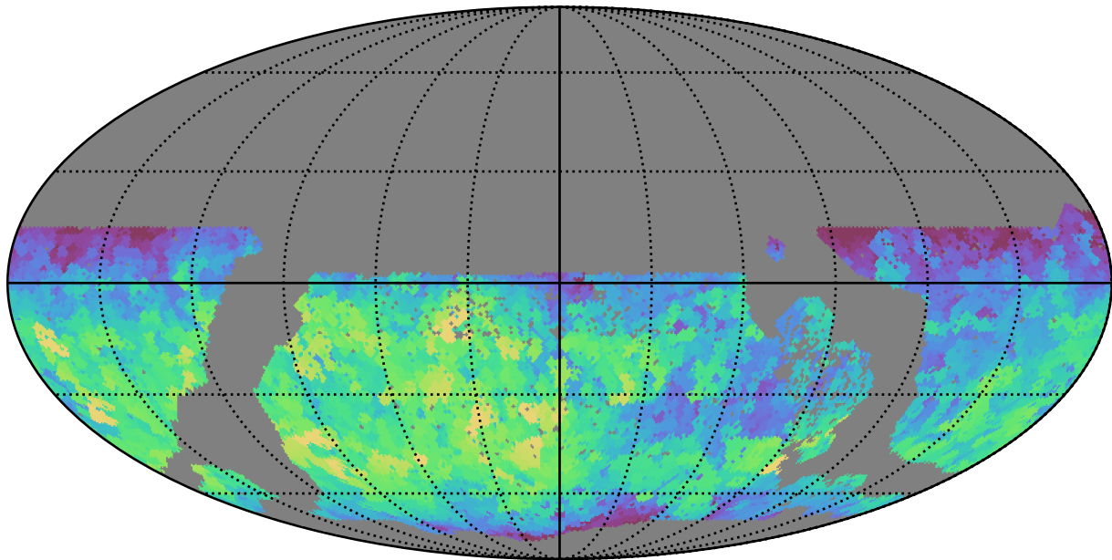
ddf_loaded_fl15_v3.4_10yrs WFD g band: Max fiveSigmaDepth
