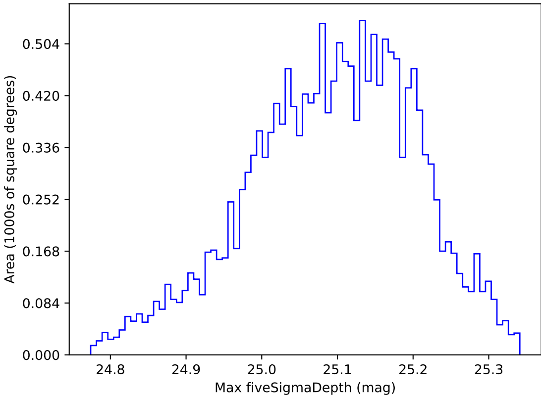
ddf_loaded_fl15_v3.4_10yrs WFD g band: Max fiveSigmaDepth
