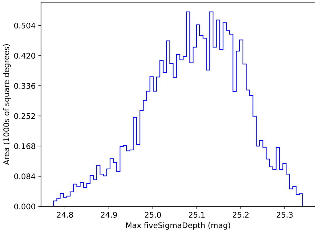
ddf_loaded_fl15_v3.4_10yrs WFD all bands: Max fiveSigmaDepth
