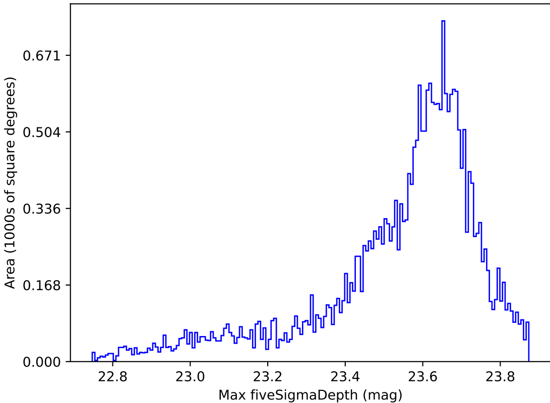
ddf_loaded_fl15_v3.4_10yrs All sky z band: Max fiveSigmaDepth
