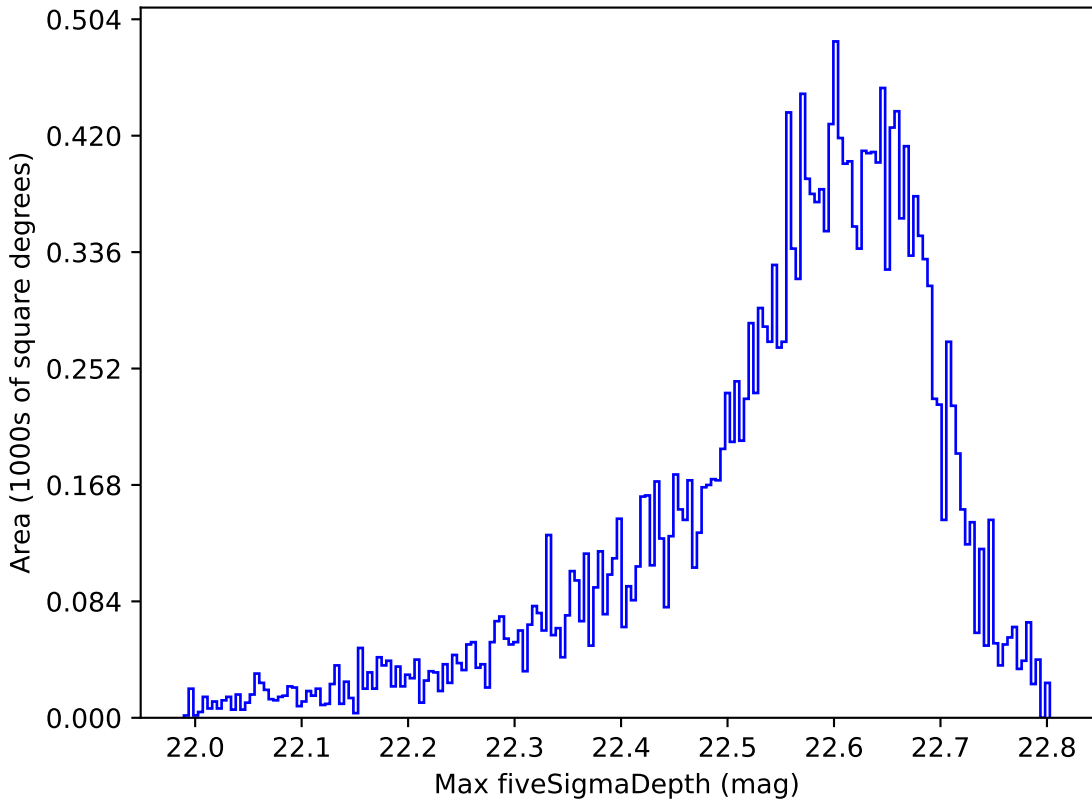
ddf_loaded_fl15_v3.4_10yrs All sky y band: Max fiveSigmaDepth
