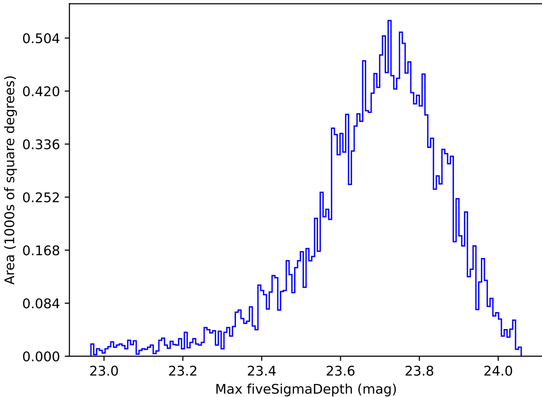
ddf_loaded_fl15_v3.4_10yrs All sky u band: Max fiveSigmaDepth
