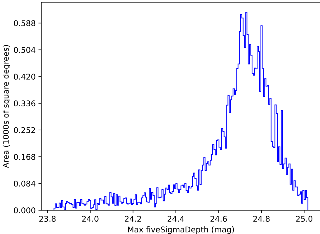
ddf_loaded_fl15_v3.4_10yrs All sky r band: Max fiveSigmaDepth
