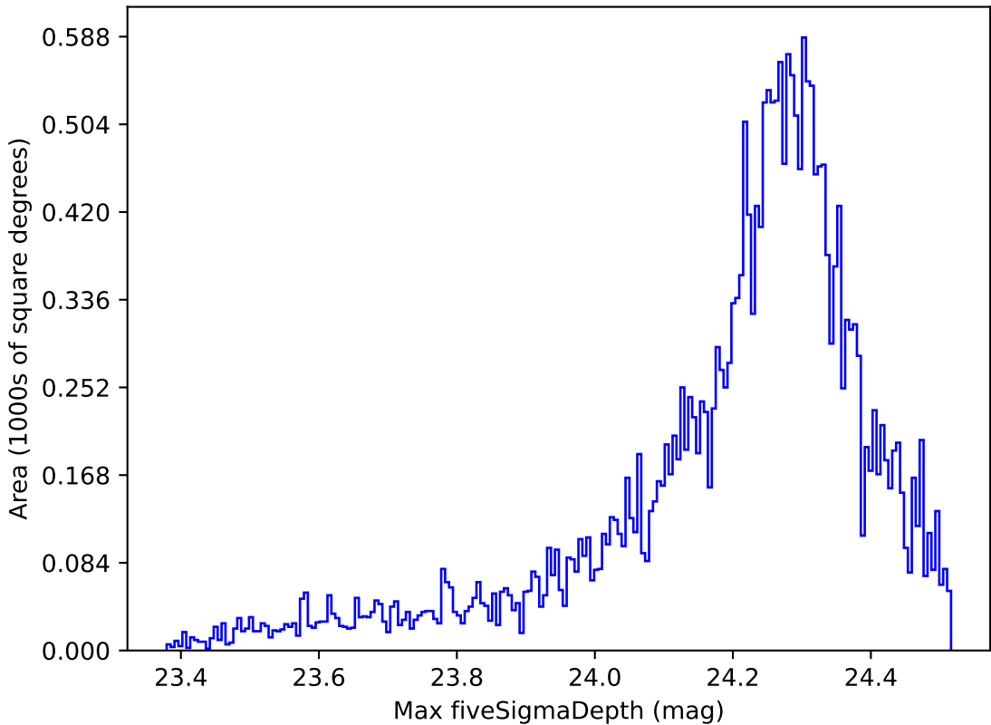
ddf_loaded_fl15_v3.4_10yrs All sky i band: Max fiveSigmaDepth
