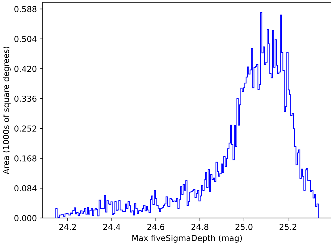
ddf_loaded_fl15_v3.4_10yrs All sky g band: Max fiveSigmaDepth
