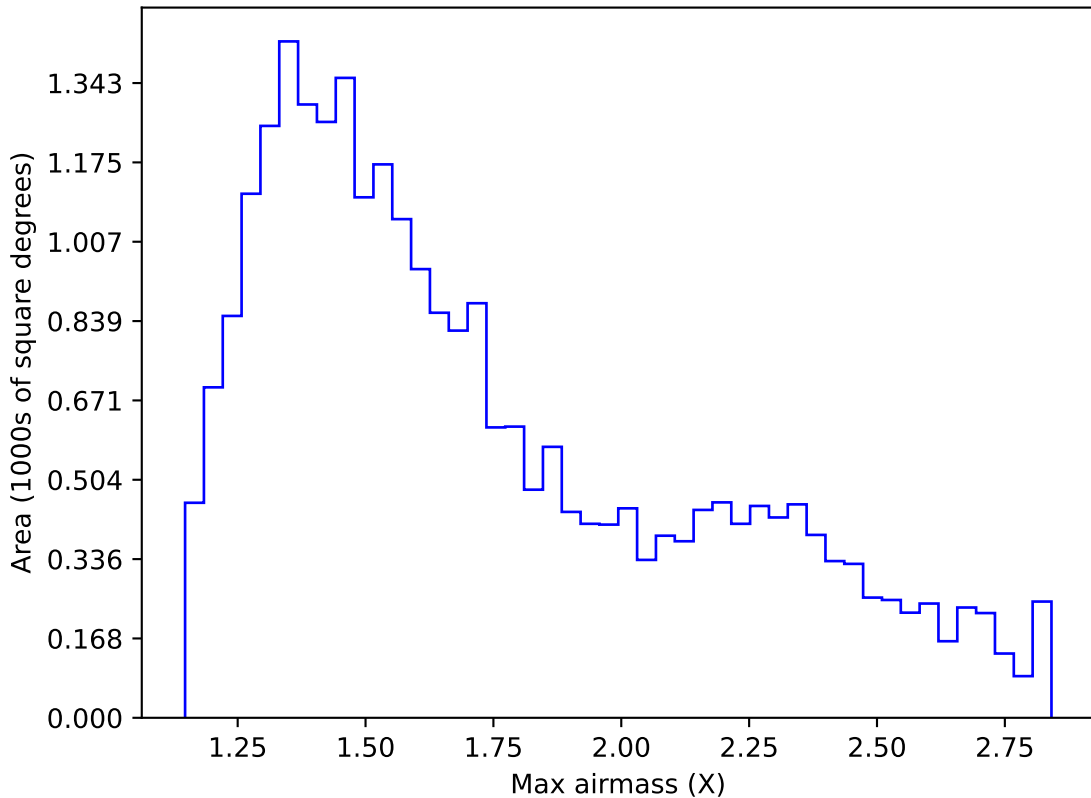
ddf_loaded_fl15_v3.4_10yrs Yr 1 z band: Max airmass
