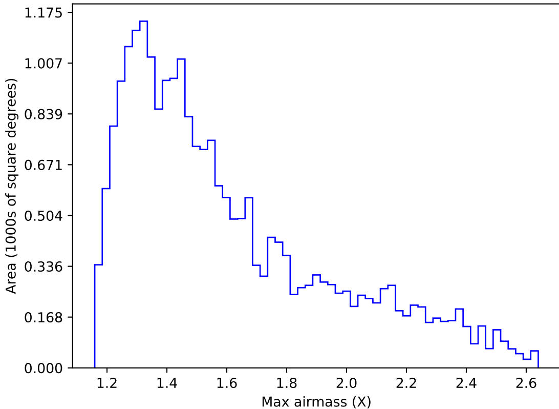
ddf_loaded_fl15_v3.4_10yrs Yr 1 y band: Max airmass
