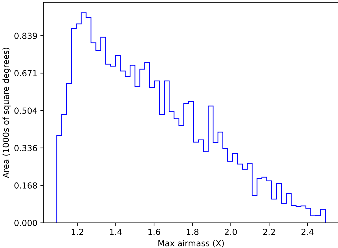
ddf_loaded_fl15_v3.4_10yrs Yr 1 u band: Max airmass
