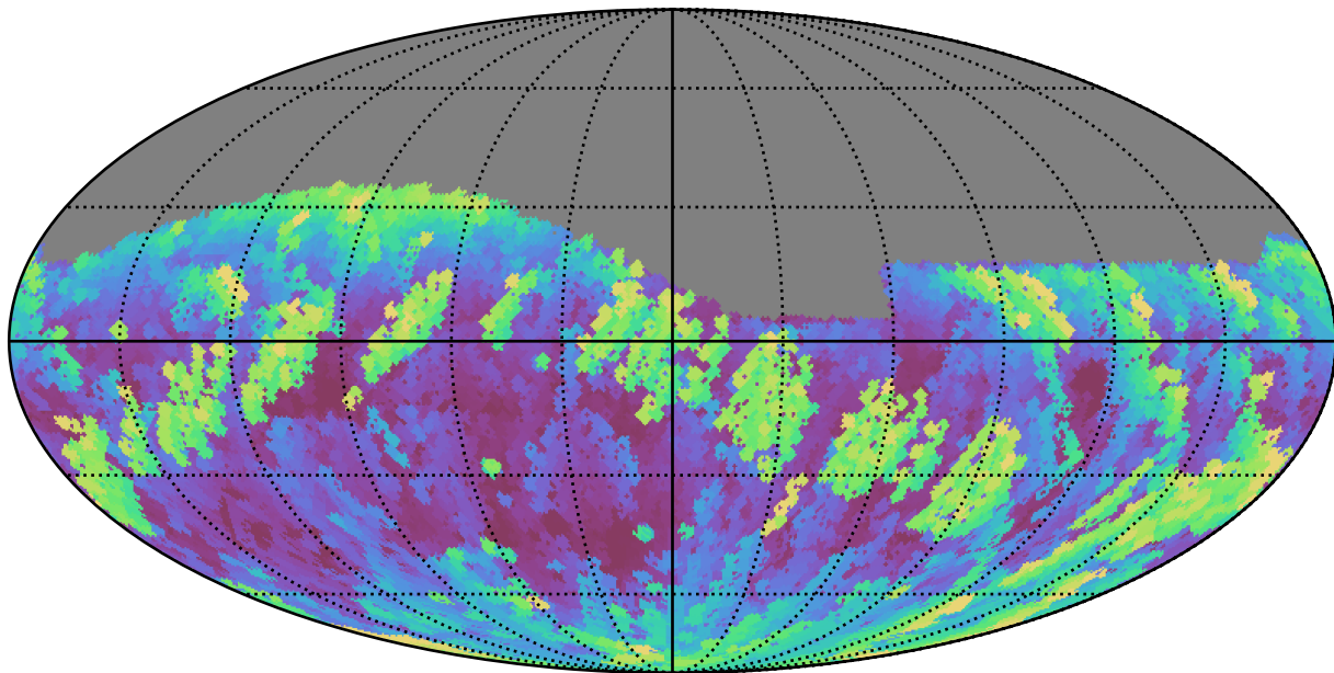
ddf_loaded_fl15_v3.4_10yrs Yr 1 r band: Max airmass
