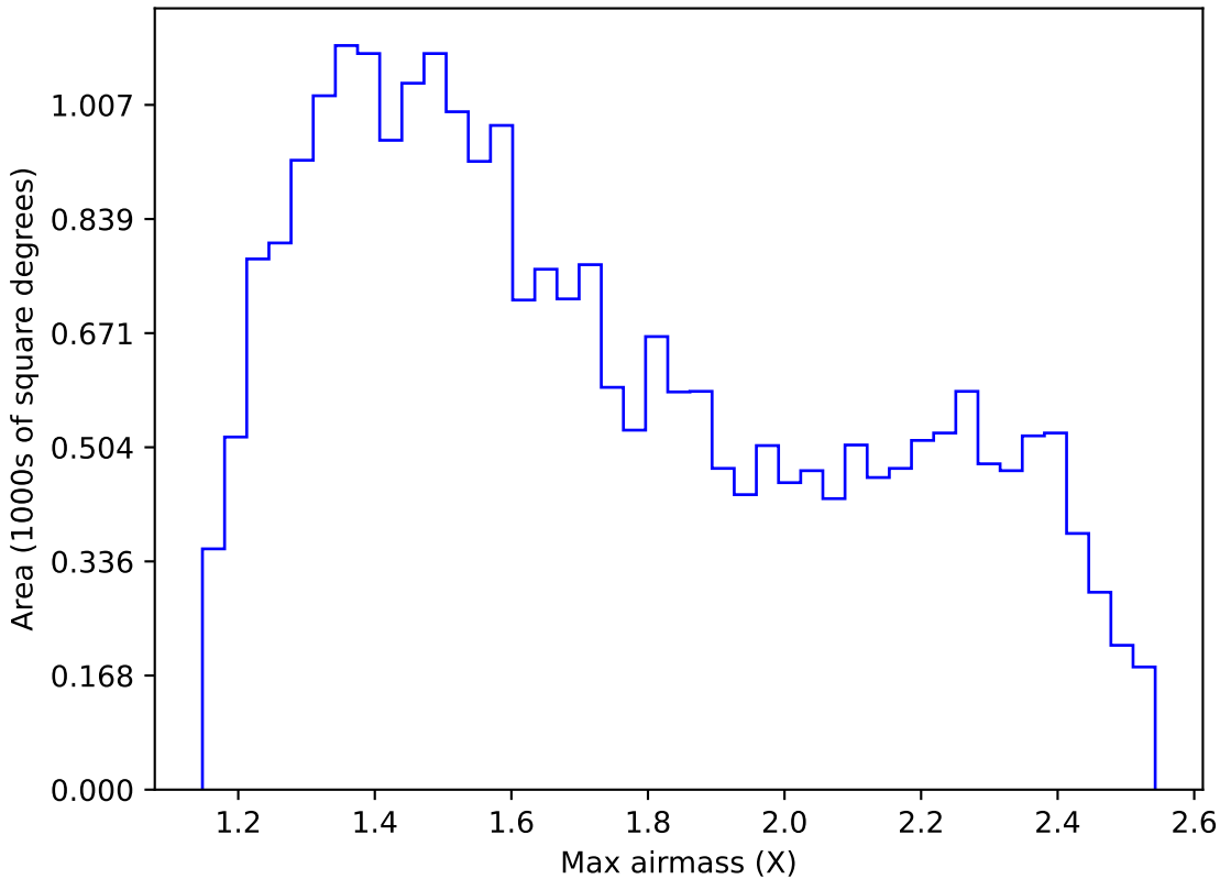
ddf_loaded_fl15_v3.4_10yrs Yr 1 r band: Max airmass
