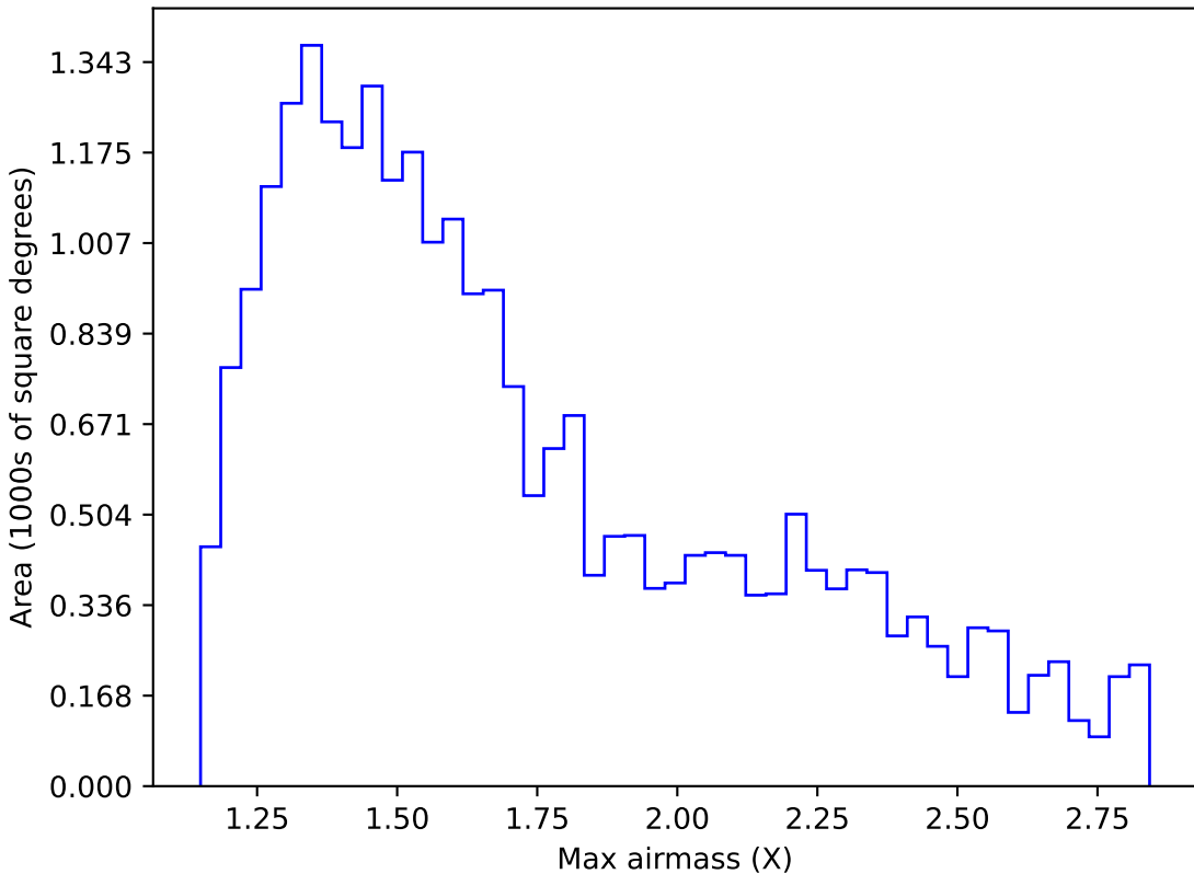
ddf_loaded_fl15_v3.4_10yrs Yr 1 i band: Max airmass
