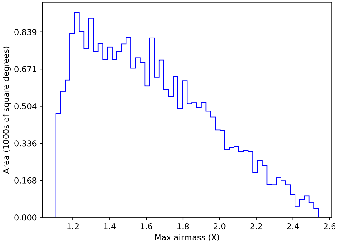
ddf_loaded_fl15_v3.4_10yrs Yr 1 g band: Max airmass
