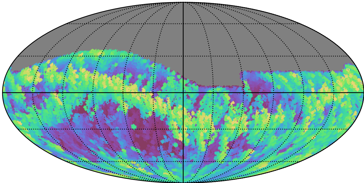
ddf_loaded_fl15_v3.4_10yrs Yr 1 all bands: Max airmass
