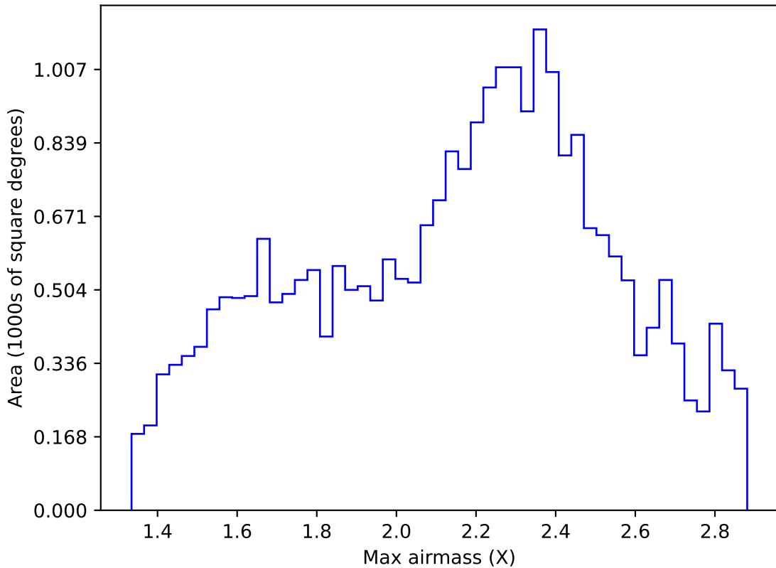
ddf_loaded_fl15_v3.4_10yrs Yr 1 all bands: Max airmass
