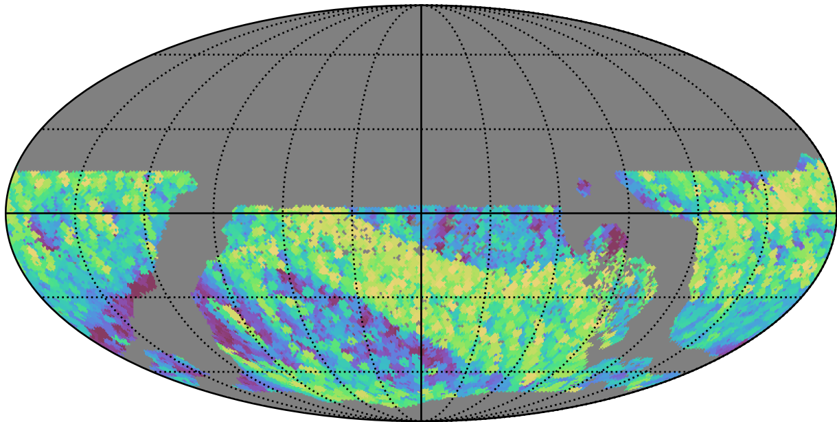
ddf_loaded_fl15_v3.4_10yrs WFD z band: Max airmass
