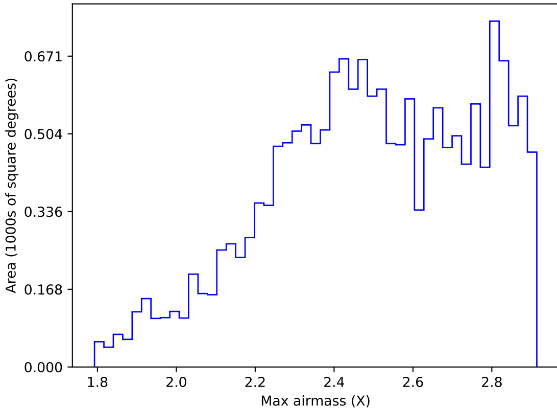
ddf_loaded_fl15_v3.4_10yrs WFD z band: Max airmass
