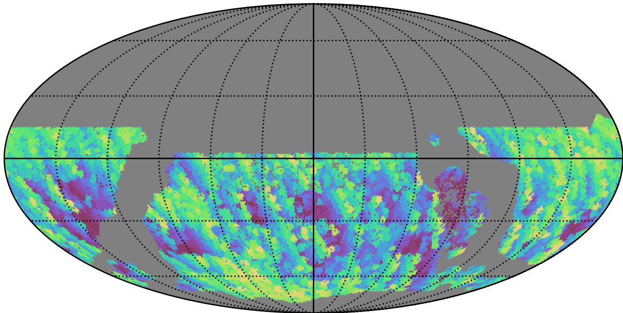
ddf_loaded_fl15_v3.4_10yrs WFD y band: Max airmass
