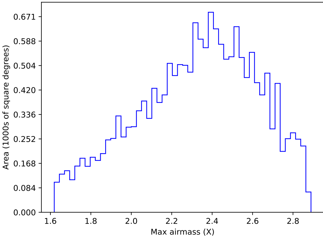
ddf_loaded_fl15_v3.4_10yrs WFD y band: Max airmass
