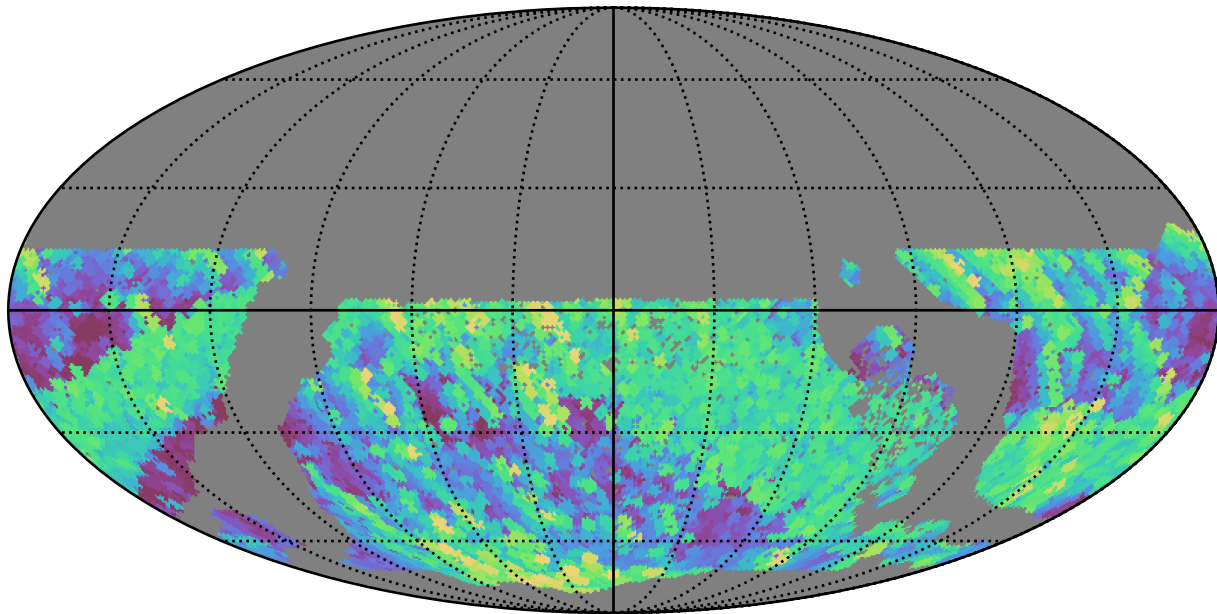
ddf_loaded_fl15_v3.4_10yrs WFD r band: Max airmass
