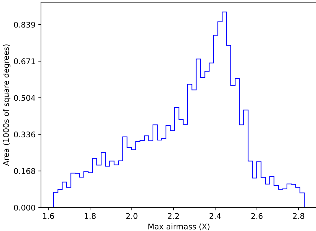
ddf_loaded_fl15_v3.4_10yrs WFD r band: Max airmass
