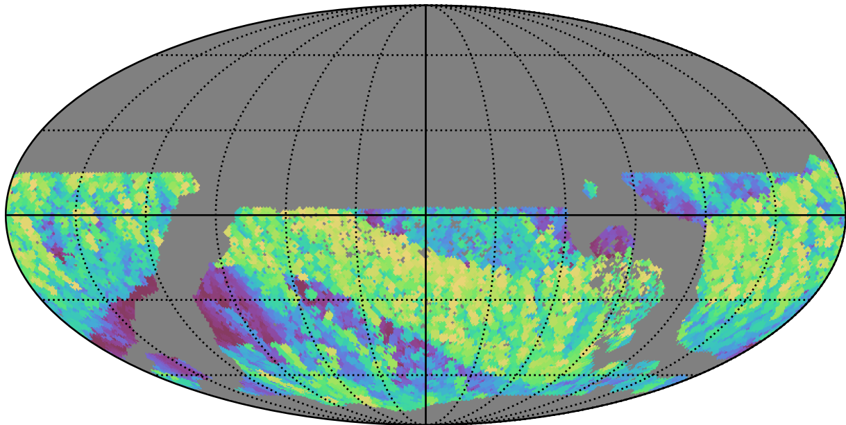
ddf_loaded_fl15_v3.4_10yrs WFD i band: Max airmass
