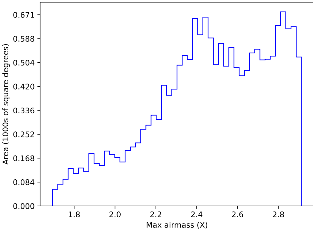
ddf_loaded_fl15_v3.4_10yrs WFD i band: Max airmass
