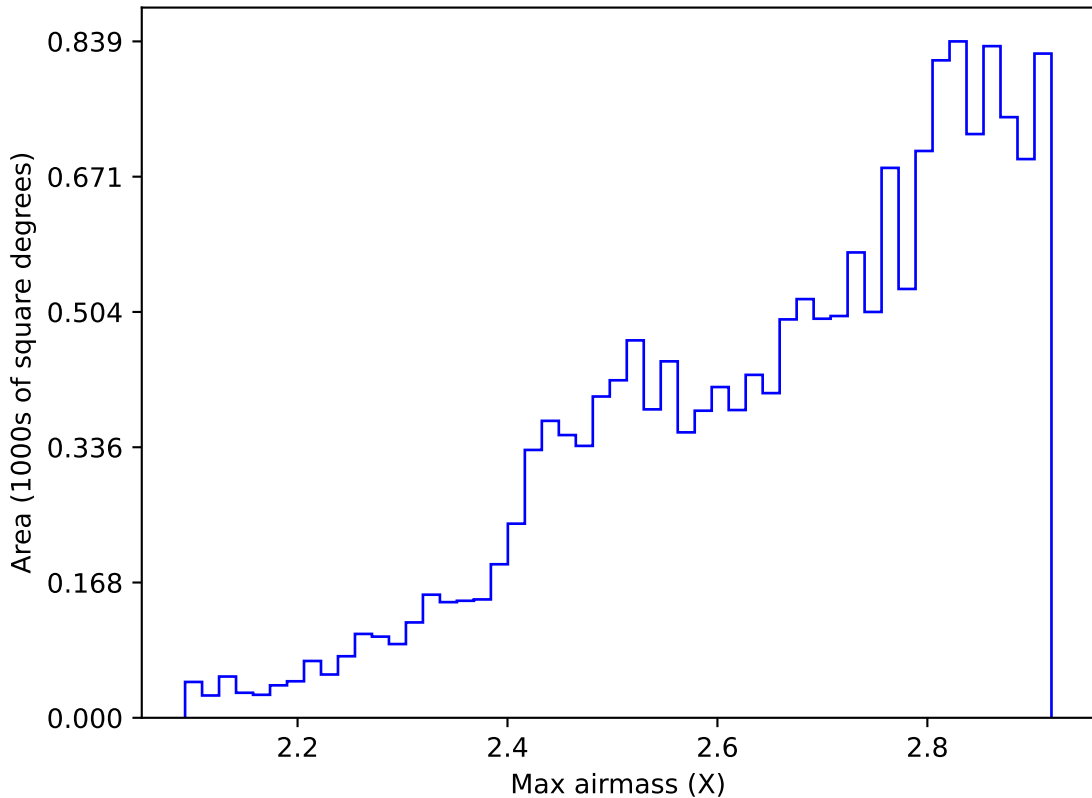
ddf_loaded_fl15_v3.4_10yrs WFD all bands: Max airmass
