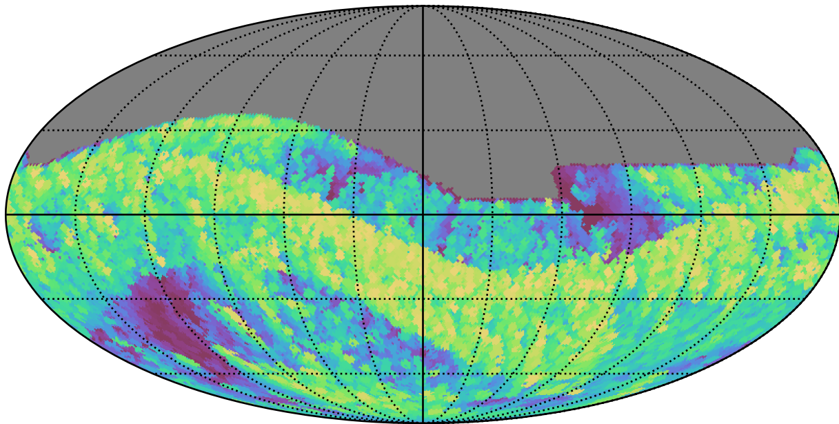
ddf_loaded_fl15_v3.4_10yrs All sky z band: Max airmass
