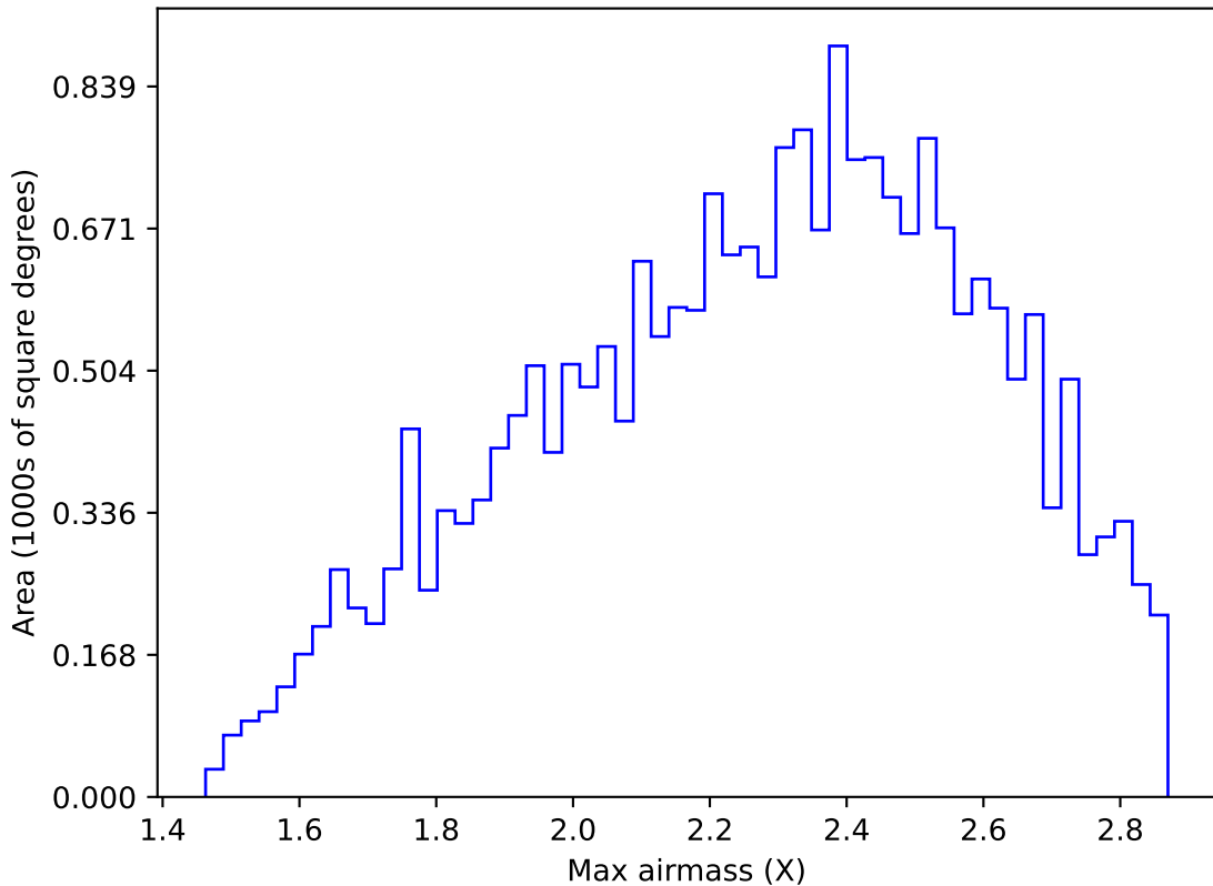
ddf_loaded_fl15_v3.4_10yrs All sky y band: Max airmass
