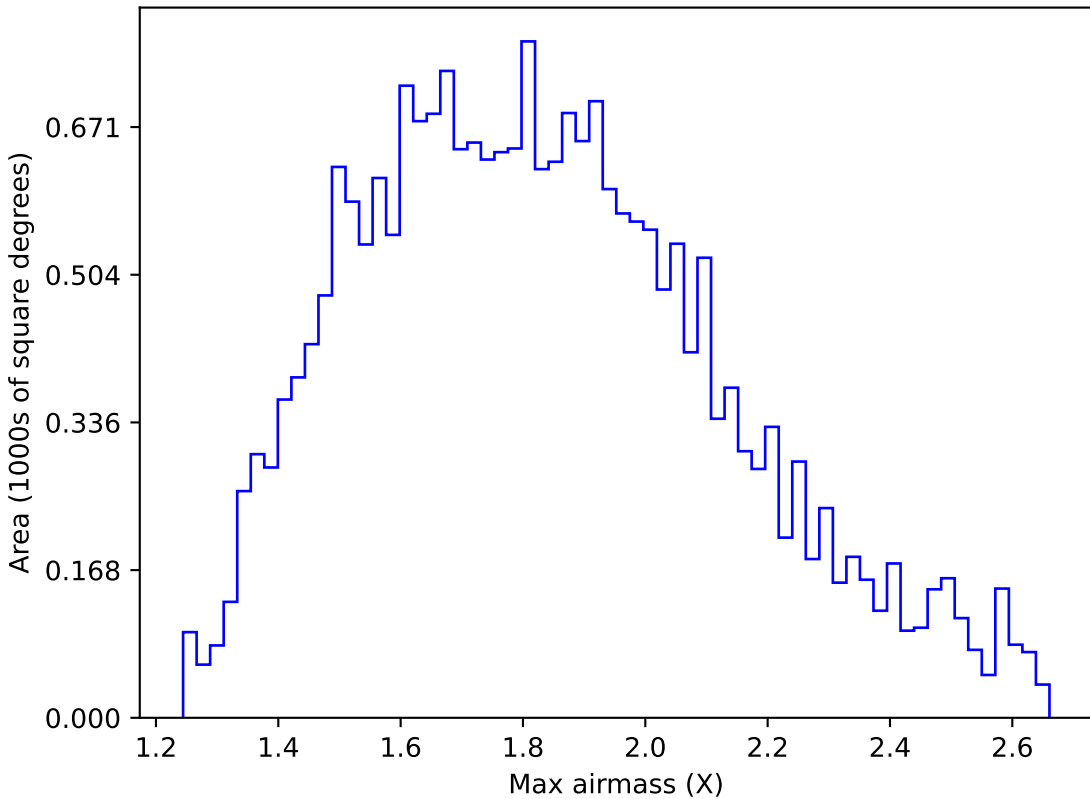
ddf_loaded_fl15_v3.4_10yrs All sky u band: Max airmass
