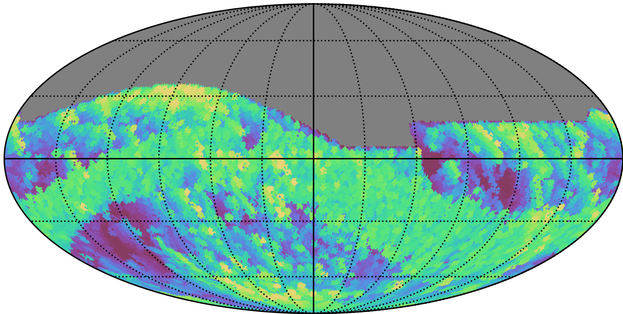
ddf_loaded_fl15_v3.4_10yrs All sky r band: Max airmass
