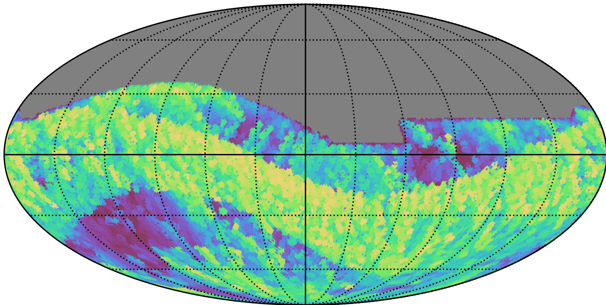
ddf_loaded_fl15_v3.4_10yrs All sky i band: Max airmass
