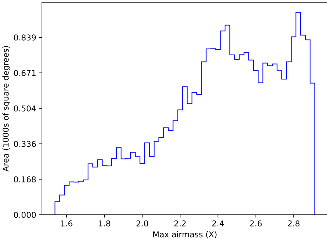
ddf_loaded_fl15_v3.4_10yrs All sky i band: Max airmass
