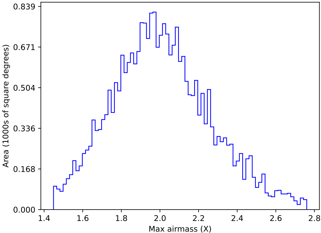
ddf_loaded_fl15_v3.4_10yrs All sky g band: Max airmass
