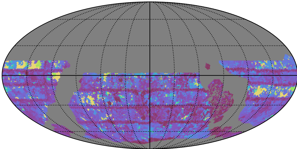
ddf_loaded_fl15_v3.4_10yrs WFD z band: Max Inter-Night Gap
