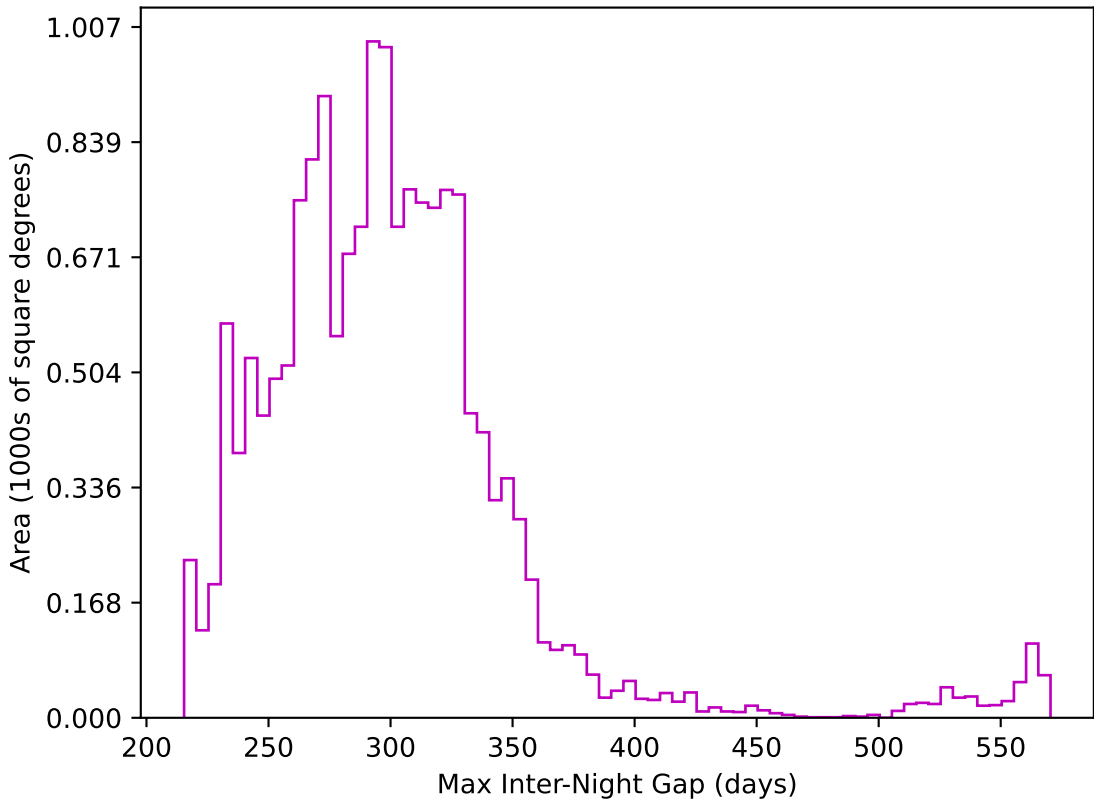
ddf_loaded_fl15_v3.4_10yrs WFD z band: Max Inter-Night Gap
