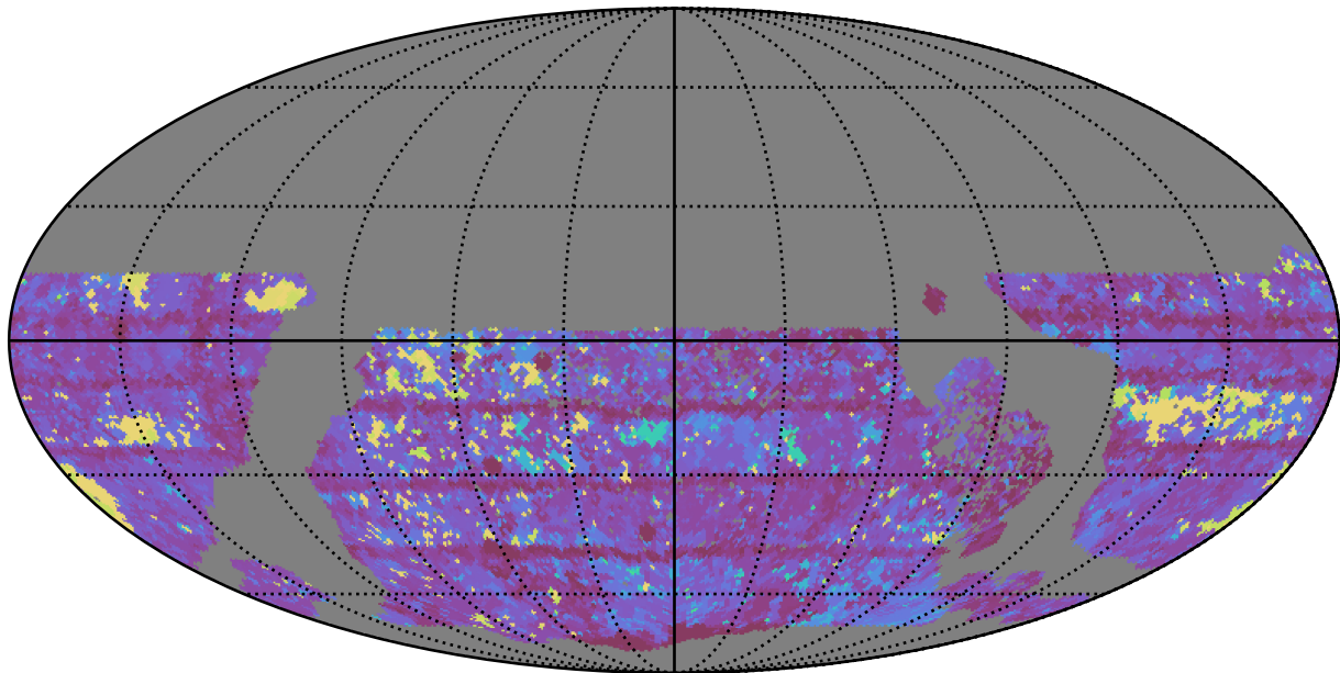
ddf_loaded_fl15_v3.4_10yrs WFD y band: Max Inter-Night Gap
