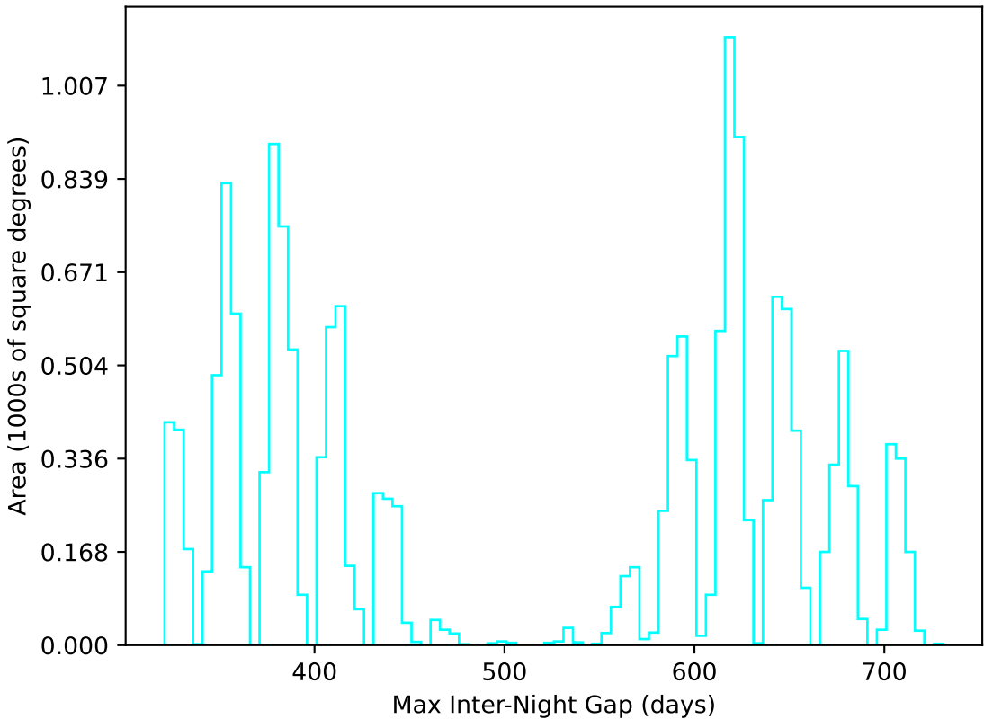
ddf_loaded_fl15_v3.4_10yrs WFD u band: Max Inter-Night Gap
