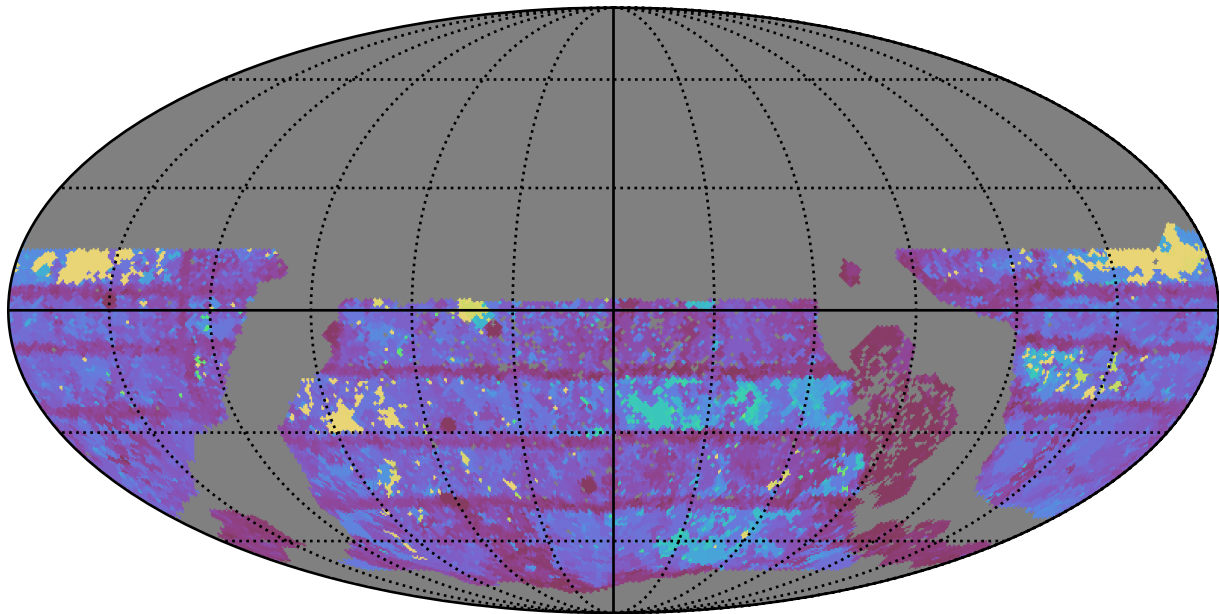
ddf_loaded_fl15_v3.4_10yrs WFD r band: Max Inter-Night Gap
