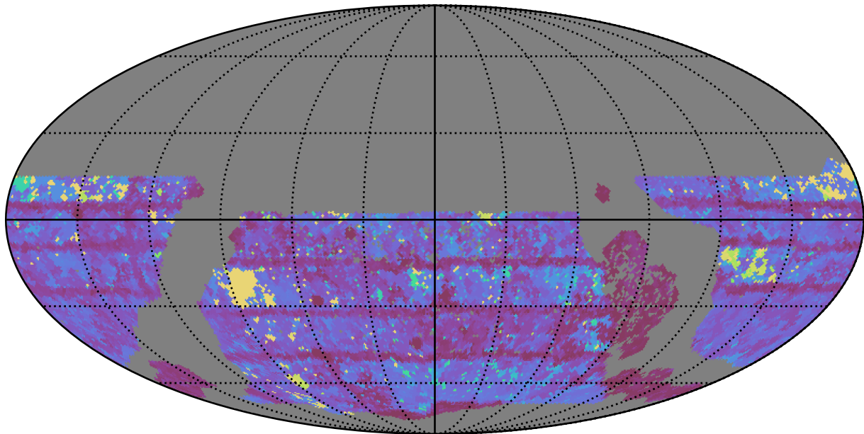
ddf_loaded_fl15_v3.4_10yrs WFD i band: Max Inter-Night Gap
