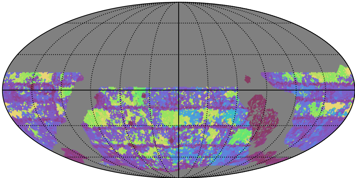
ddf_loaded_fl15_v3.4_10yrs WFD g band: Max Inter-Night Gap
