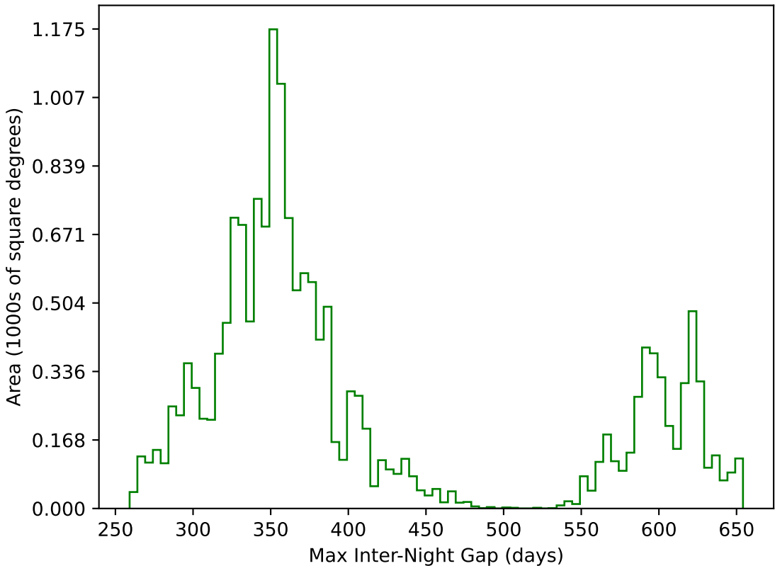
ddf_loaded_fl15_v3.4_10yrs WFD g band: Max Inter-Night Gap
