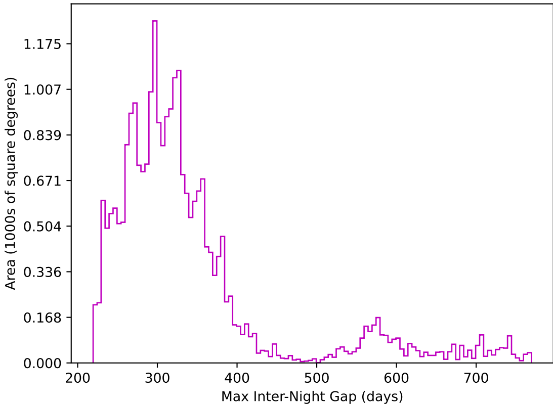
ddf_loaded_fl15_v3.4_10yrs All sky z band: Max Inter-Night Gap
