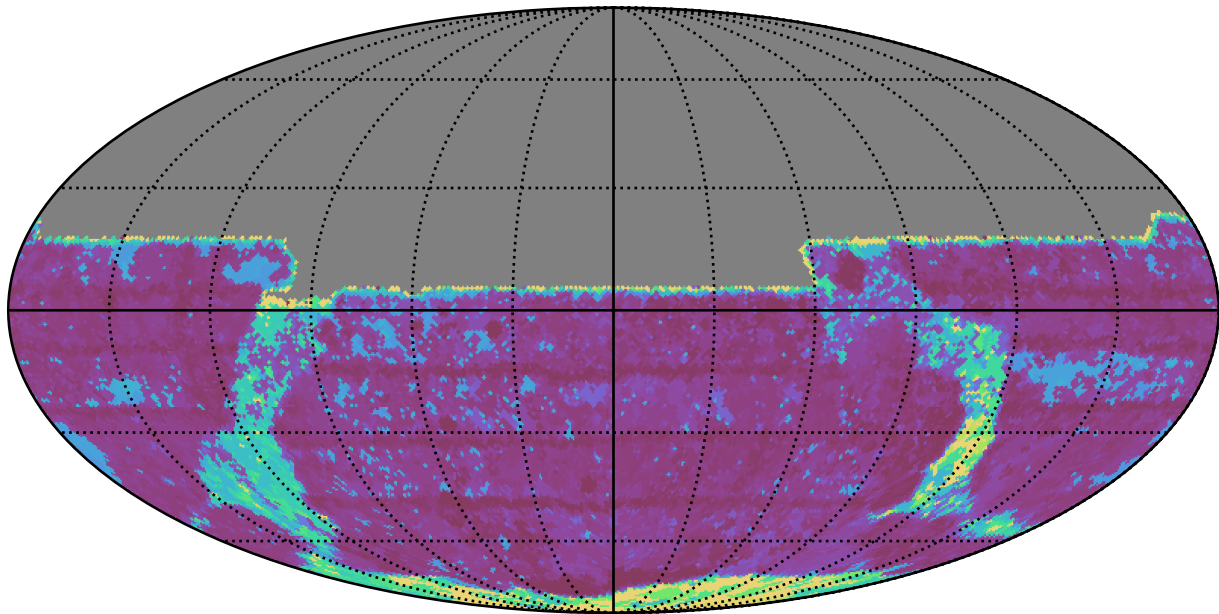
ddf_loaded_fl15_v3.4_10yrs All sky y band: Max Inter-Night Gap
