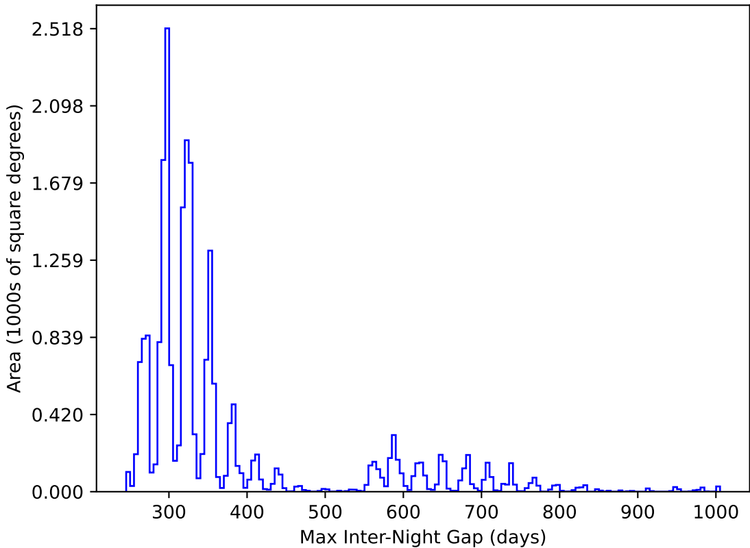
ddf_loaded_fl15_v3.4_10yrs All sky y band: Max Inter-Night Gap
