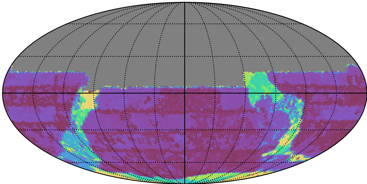
ddf_loaded_fl15_v3.4_10yrs All sky u band: Max Inter-Night Gap
