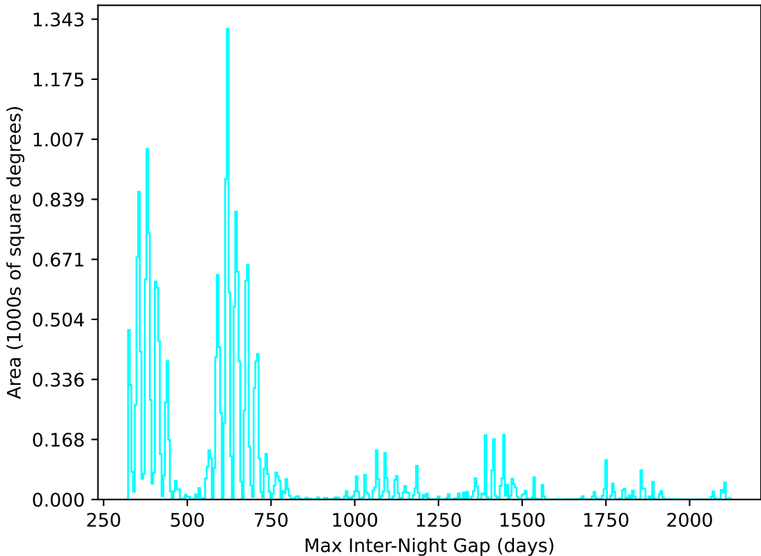
ddf_loaded_fl15_v3.4_10yrs All sky u band: Max Inter-Night Gap
