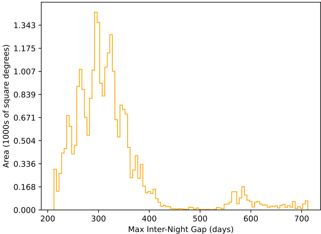
ddf_loaded_fl15_v3.4_10yrs All sky r band: Max Inter-Night Gap
